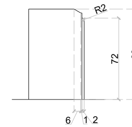
A'-A SECTION
