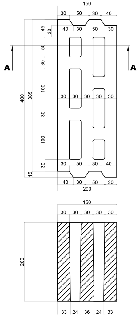
OPEN BLOCK A - A SECTION
